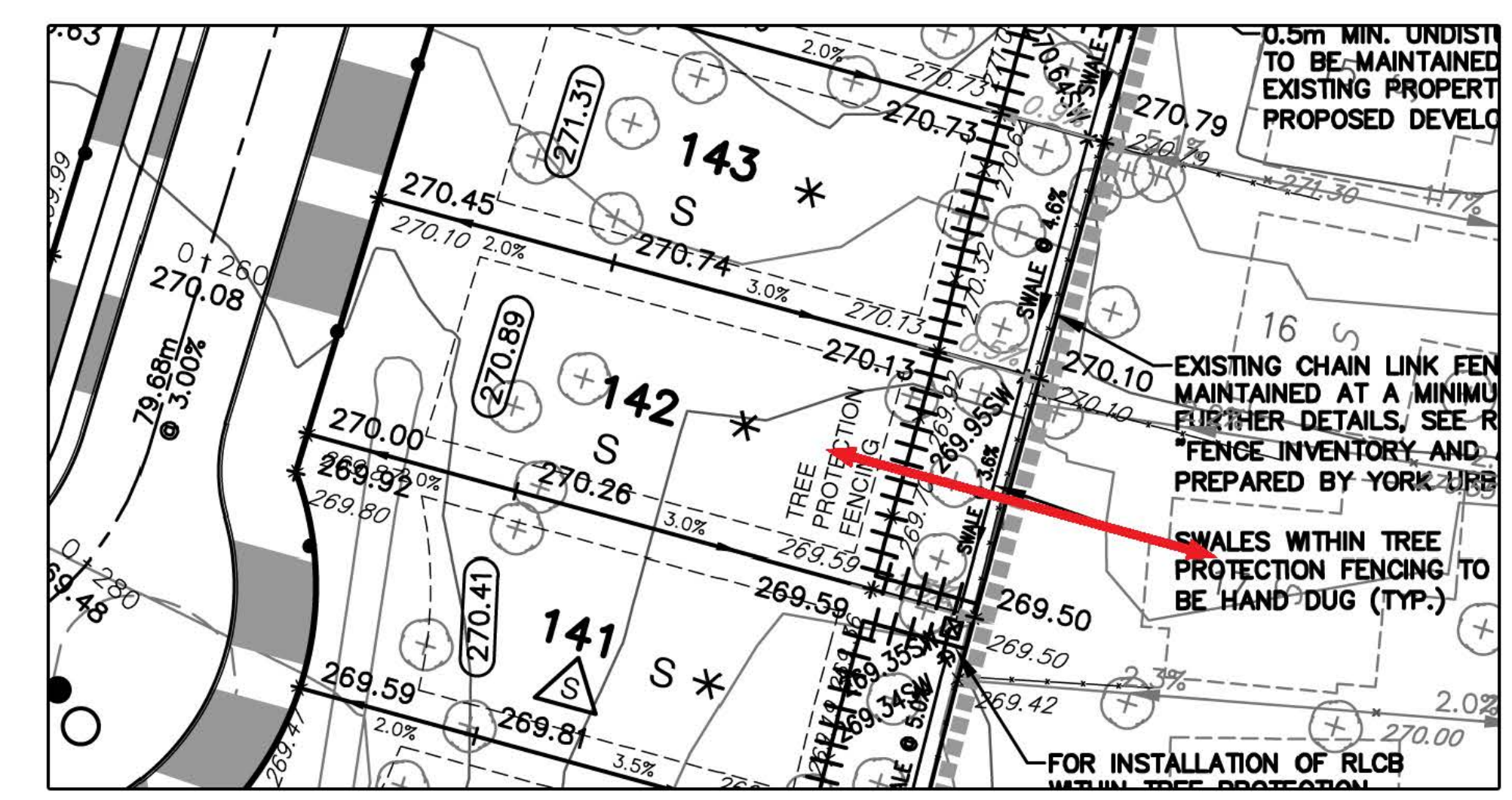
Grading Plan Excerpt - Lot 142
