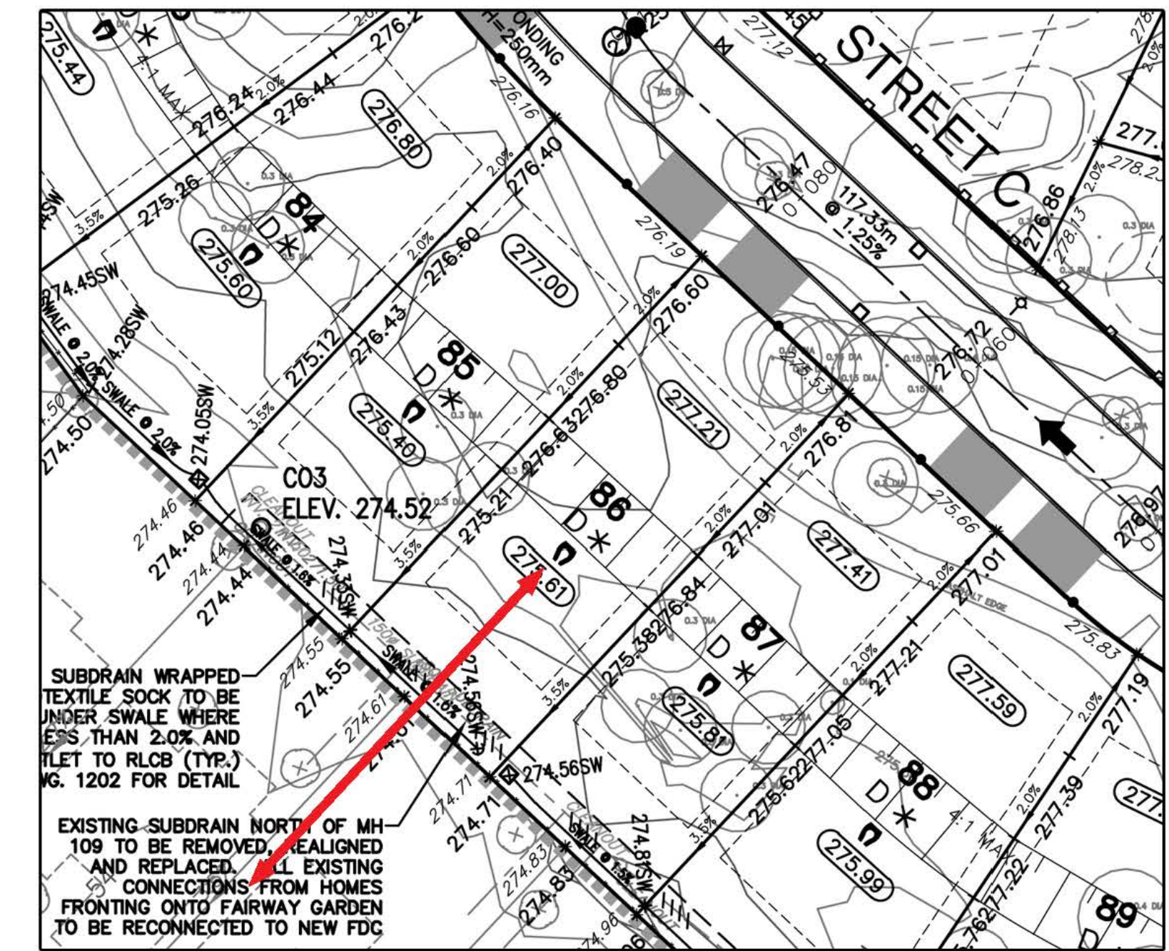
Grading Plan Excerpt - Lot 86
